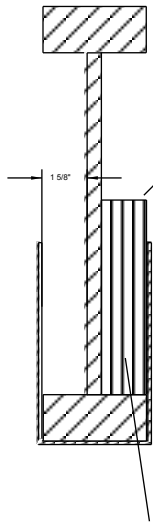
Blocking example one side front view (Block both sides equally)
